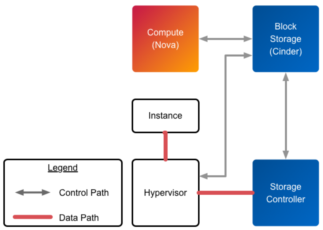
Figure 4.1. Cinder and Nova Logical Architecture
